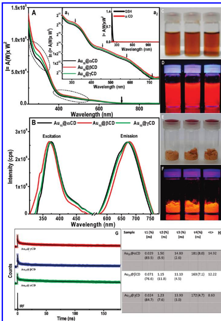
Figure 1. (A) UV-vis spectra of Au 15 @ \alpha CD, Au 15 @ \beta CD, and Au 15 @ \gamma CD clusters inside the CD cavity. Ellipses indicate the distinct features of the Au 15 core. Inset a 1 gives the plot of the natural logarithm of the Jacobian factor, versus wavelength, of all three clusters, to show the molecular features more clearly. Well-defined absorption features are marked with arrows. The threshold of absorption is also marked. Absorption profiles of pure GSH and \alpha CD are given in inset a 2 . (B) PL spectra of all three samples (375 nm excitation). (C) Photograph of the cluster solutions under white light. (D) Photograph of the cluster solutions under UV light. (E) Photograph of the three cluster powders under white light. (F) Photograph of the three cluster powders under UV light. (G) Luminescence decay of Au 15 @ \alpha CD, Au 15 @ \beta CD, and Au 15 @ \gamma CD clusters in water. (H) Table giving the lifetime values for Au 15 @ \alpha CD, Au 15 @ \beta CD, and Au 15 @ \gamma CD.
